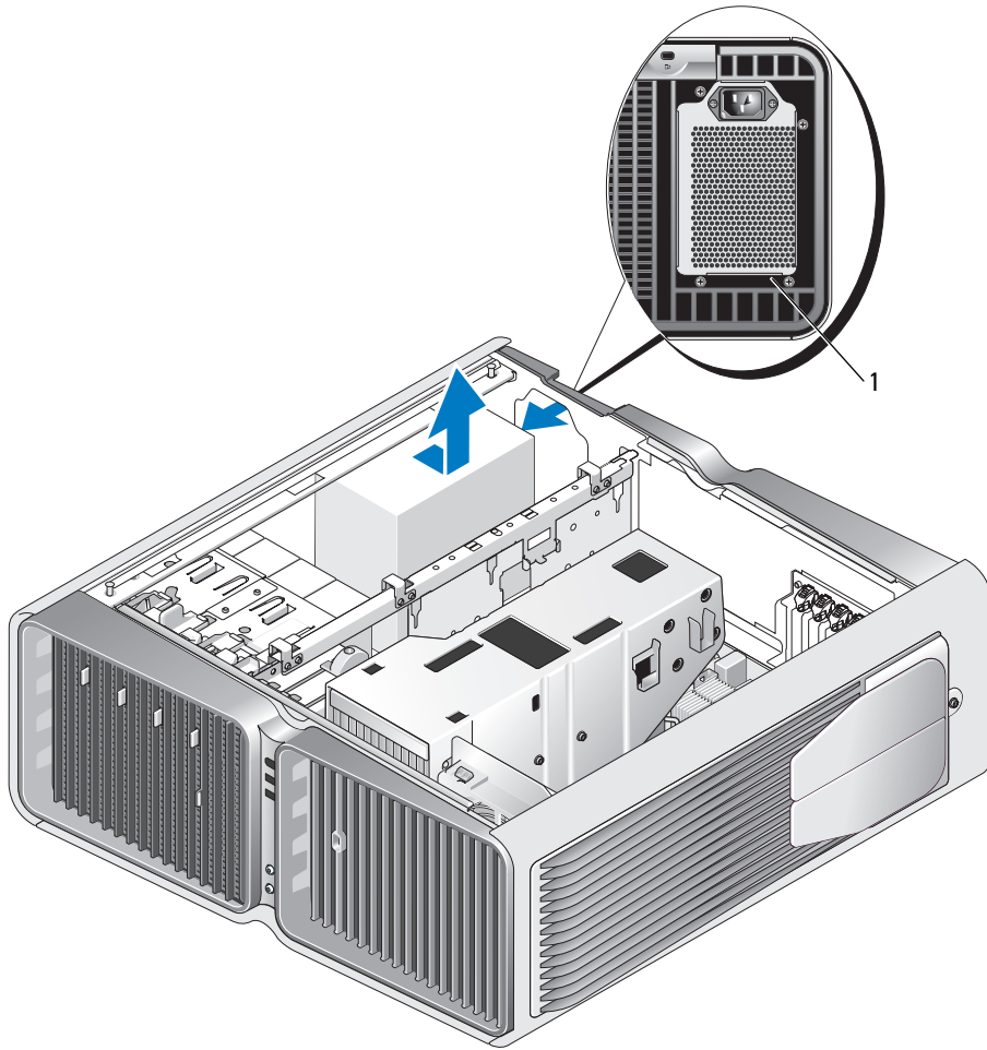
1 power supply screws (4)
