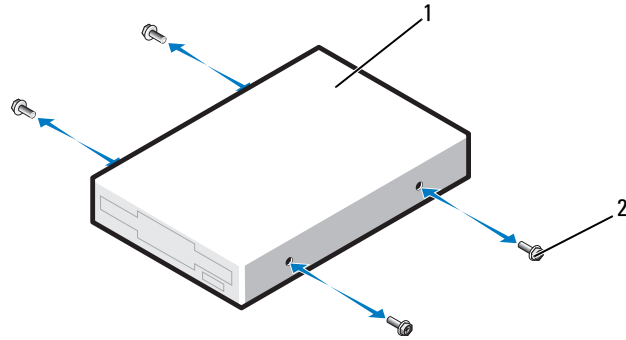
1 media card reader 2 shoulder screws (4)
