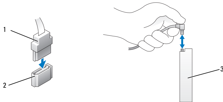
2 SATA data connector (on the system board)
